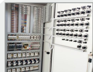
MCC Panel
